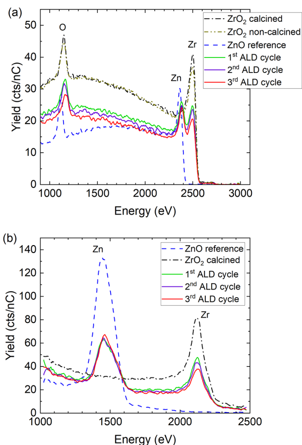
Figure 11. LEIS spectra of ZnO ALD samples deposited on \text{ZrO}_2 with different ALD cycle numbers. (a) 3 keV \text{He}^+ and (b) 5 keV \text{Ne}^+ were used as the primary ions. The LEIS spectra of the nontreated \text{ZrO}_2 , \text{ZrO}_2 calcined at 600 °C, and ZnO powder as references. In 5 keV \text{Ne}^+ spectra, only elements heavier than Ne are detected, but the mass resolution is vastly improved compared to the \text{He}^+ spectra.
