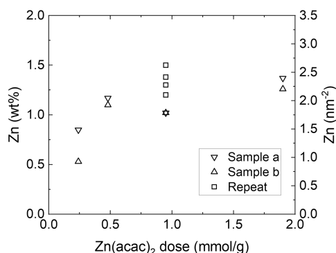
Figure 2. ICP-OES analysis of the zinc loading on \text{ZrO}_2 as a function of the \text{Zn}(\text{acac})_2 dose. An ALD temperature of 200^\circ\text{C} was used. The areal number density of zinc ( \text{nm}^{-2} ) was calculated by using a specific surface area of calcined \text{ZrO}_2 of 53.5\text{ m}^2\text{ g}^{-1} .
