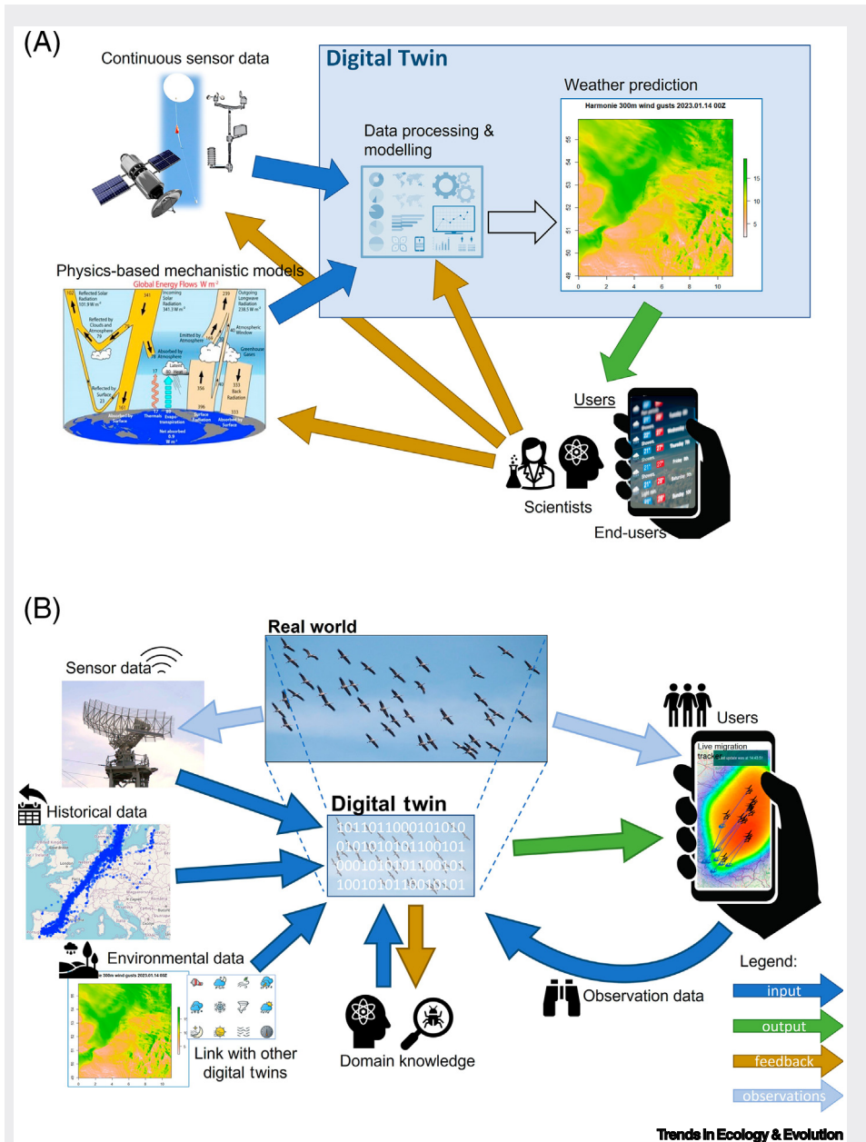
Figure I. Examples of digital twins (DTs). Established physics-based mechanistic models are used for weather forecasting (A), but due to their inherent nonlinearities, their predictions quickly become too uncertain to be useful. Model predictions are therefore continuously updated with high-resolution sensory data. (B) There is no mechanistic model for predicting crane ( Grus grus ) migration. Instead, in an empirical model sensory data from migrating cranes are combined with environmental data such as wind directions. In addition to such data, the output of environmental DTs could be used as well. Again, because predictions of routes taken by cranes quickly become uncertain, citizen science sighting data are used to update the output of the crane DT. In both examples, the design, model, and workflows underlying the DT are driven by user demand for relevant and reliable predictions.
