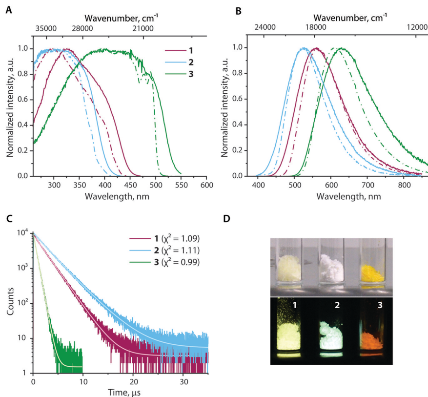
Figure 4. Normalized excitation (A) and emission (B) spectra of compounds 1–3 in the solid state at 297 K (solid line) and 77 K (dashed-dotted line); C) time-resolved and fitted decay curves at 297 K; D) images of 1–3 under ambient and UV ( \lambda_{\text{exc}}=365 nm) light.
