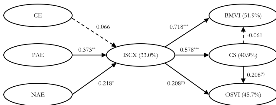
Figure 2: Model estimates (** = p < 0.01 , * = p < 0.05 , (*) = p < 0.10 )
