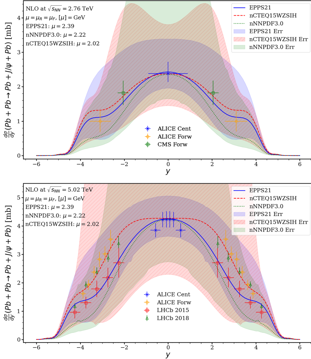
FIG. 4. The PDF uncertainties of the NLO pQCD predictions for the d\sigma(Pb + Pb \rightarrow Pb + J/\psi + Pb)/dy cross section as a function of y for Run 1 (top) and Run 2 (bottom) at the LHC, and a comparison with the corresponding Run 1 [39–41] and Run 2 [42–45] data, mirrored with respect to y = 0 and with the statistical and systematic errors added in quadrature. The results corresponding to the central sets of nPDFs are shown by the blue solid (EPPS21), red dashed (nCTEQ15WZSIH), and green dotted (nNNPDF3.0) curves, respectively, and the error bands are represented by the corresponding shaded regions. All calculations are performed at the indicated values of the optimal scale \mu .
