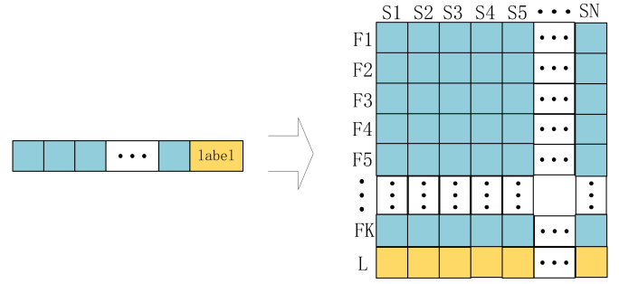
Fig. 3: Feature recombination for encoder
