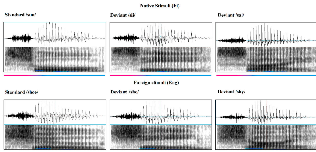
Figure 1. Spectrograms of the stimuli used in the oddball paradigm. At the top are the native (Finnish) stimuli and at the bottom are the foreign (English) stimuli. The color bar below shows the sound change from the fricative (in pink) to vowel(s) (in blue) at around 120 ms.
