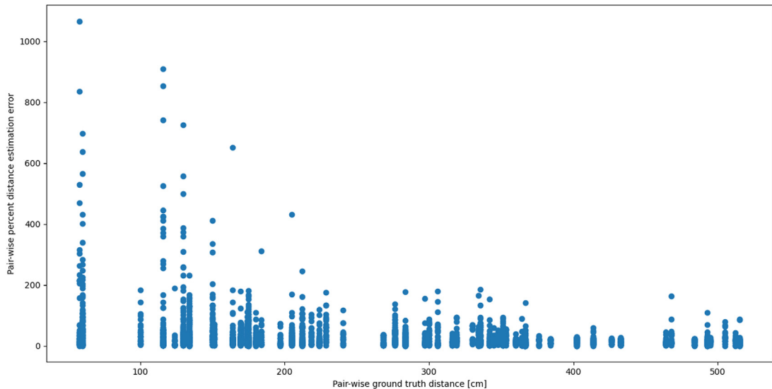
Fig. 11. Pair-wise distance estimation errors for each of the ground truth pair-wise distances.
