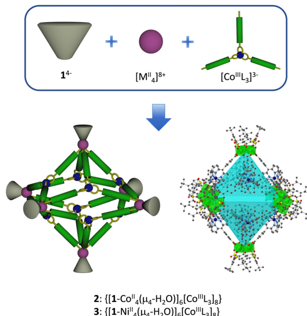
Fig. 2 The three-component approach leading to the formation of octahedral cages 2 and 3 . On the bottom, the representation of a cage from X-ray diffraction data. M^{II} cations in the [1-M^{II}_4(\mu_4-H_2O)]^{4+} species are represented as green polyhedra and the faces of the octahedron are colored in blue. The ( Co^{III}L_3 ) 3– connectors are located above the faces of the octahedron.
