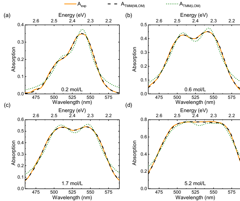
Fig. 3. Absorption profiles of the R6G films in the spectral range of the local excitonic band of interest for target concentrations: (a) 0.2 mol/L, (b) 0.6 mol/L, (c) 1.7 mol/L and (d) 5.2 mol/L. In the figure, A_{\text{TMM(LOM)}} and A_{\text{TMM(MLOM)}} represent the absorption profiles computed by TMM using the optical constants calculated from LOM and MLOM, respectively, while A_{\text{exp}} depicts the experimental (smoothed) absorption spectra.
