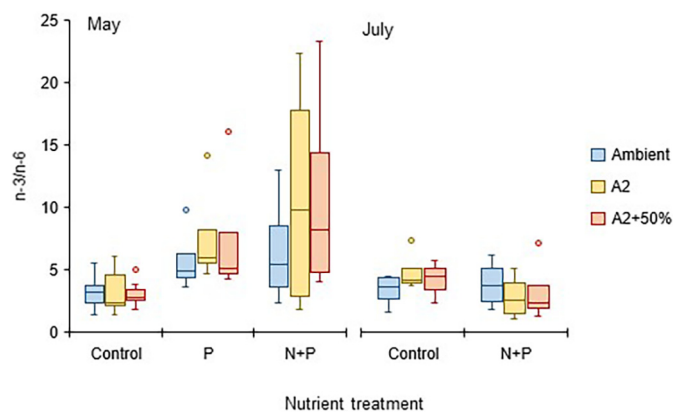
Fig. 4. Sestion n-3/n-6 ratio in May and July in mesocosm with different nutrient treatments: control, i.e., low nutrient condition, and P or N + P additions and climate scenarios.
