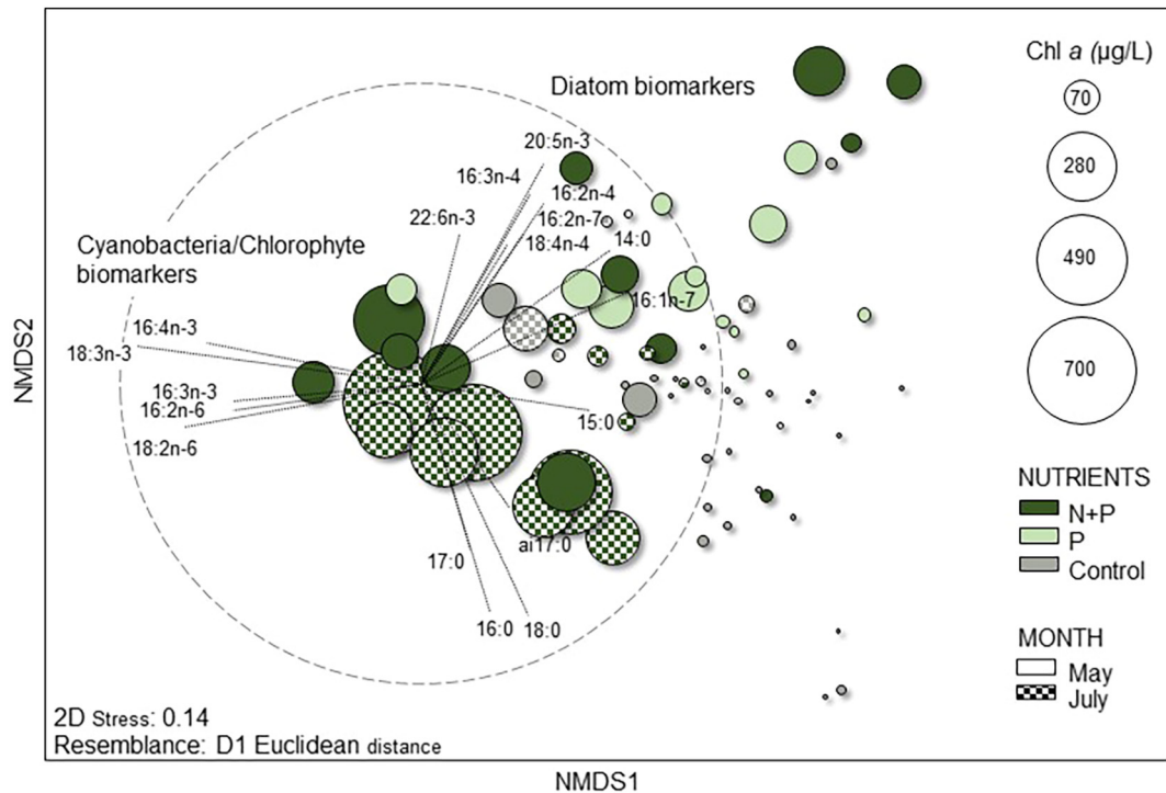
Fig. 3. NMDS based on sestion fatty acid profiles (w%). Vector overlays indicate the strength of the relationship between the variables and the NMDS axes.
