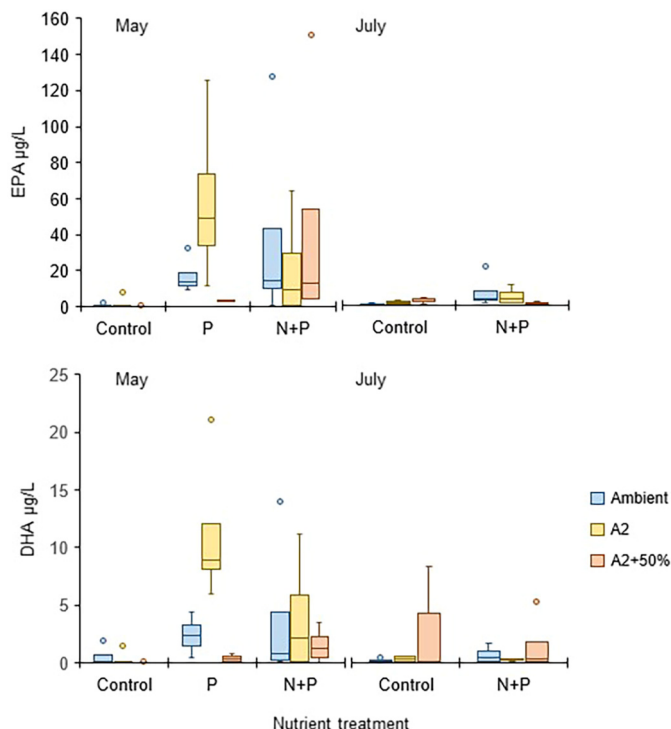
Fig. 1. Phytoplankton concentrations (µg/L) of A) EPA and B) DHA in mesocosms with different nutrient treatments: control, i.e., low nutrient condition, and P or N + P addition and climate scenarios (Ambient, A2 and A2 + 50 %). Panels refer to spring (May) and summer (July) sampling.
