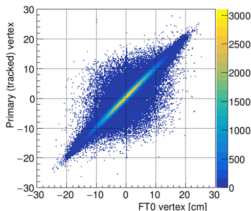
Fig. 7. Correlation between collision vertex reconstructed by the tracking detectors and FT0.
