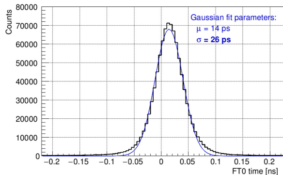
Fig. 4. FT0 collision time resolution.
