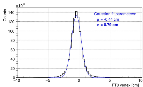
Fig. 6. FT0 vertex resolution.
