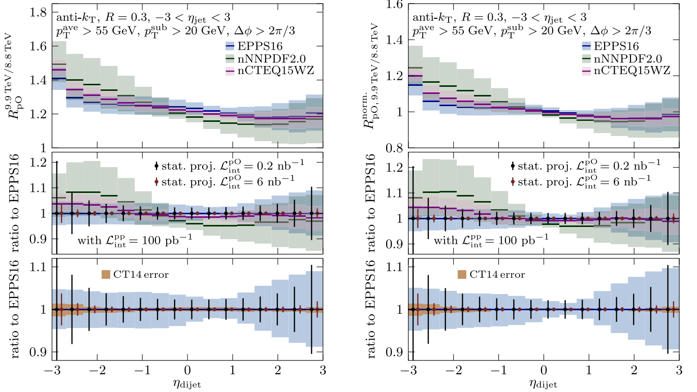
FIG. 5. As Fig. 3, but for the mixed-energy nuclear-modification ratio (left), and for the self-normalized double ratio (right).
