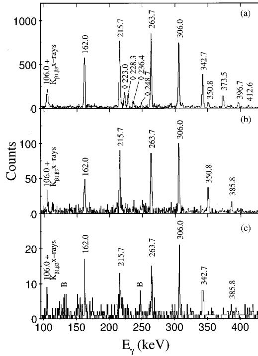
FIG. 2. \gamma spectra showing the evolution of bands 1 and 3 with increasing spin. (a) The projection of \gamma rays observed in coincidence with two or more further \gamma rays two of which must be members of the transition-energy list A (see Table I). (b) The projection of \gamma rays observed in coincidence with further two or more \gamma rays of which one must be a member of the transition-energy list A and another a 228.3-keV \gamma ray. (c) The projection of \gamma rays observed in coincidence with two or more further \gamma rays of which one must be a member of the transition-energy list A and another a 236.4-keV \gamma ray. The symbol \diamond is used to denote interband transitions and the label B denotes a background peak.
