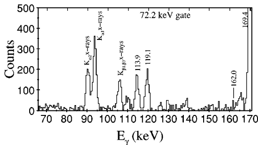
FIG. 6. Projection of \gamma rays in triple coincidence with \gamma rays of 72.2 keV. The absence of a 162.0-keV peak is indicated.
