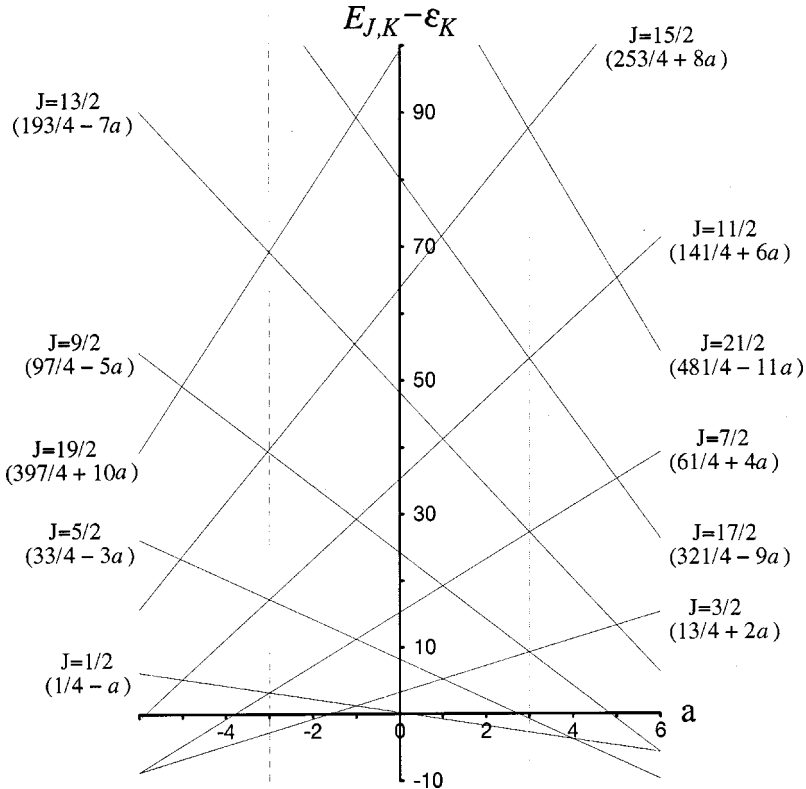
FIG. 10. Level energies in a K = 1/2 band plotted against decoupling parameter a . The term in parentheses corresponds to the value of [J(J+1) - 2K^2 + (J+1/2)a(-1)^{J+(1/2)}] [see Eq. (2)]. The vertical dashed lines represent the decoupling parameters predicted by Liang et al. as discussed in the text.
