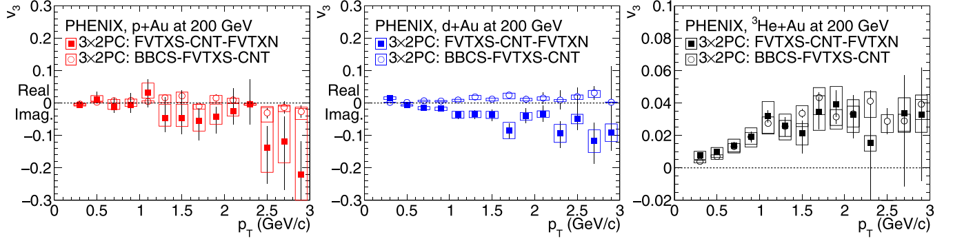
FIG. 7. The extracted v_3 coefficients as a function of p_T in 0%–5% central p + Au , d + Au , and {}^3\text{He} + Au collisions from the 3 \times 2PC method using the FVTXS-CNT-FVTXN detector combination are shown as solid squares. For comparison we also show the previously plotted results from the BBCS-FVTXS-CNT combination as open circles.
