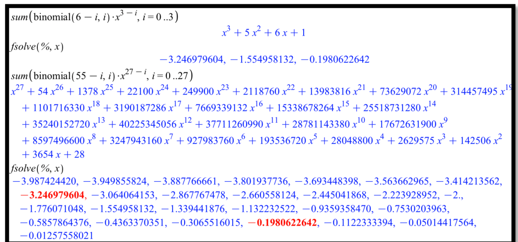
Figure 8. Illustrating Conjectures 1 and 2 when k = 7 and n = 3 .
