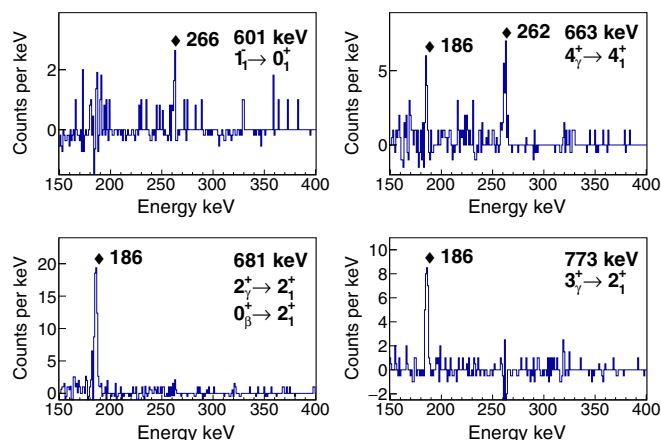
FIG. 6. Background-subtracted \gamma -ray spectra observed in time-coincidence with other \gamma -ray transitions. The energy gate is labeled corresponding to the energies, spin, and parity of the initial and final states of the relevant transition. The transitions observed in coincidence with the gate are labeled with their energy given in keV. The spectra were obtained by sorting the data in the segment mode.
