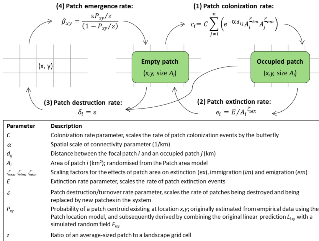
Fig. 2. States, events and event rates of the Stochastic Patch Occupancy Model in a dynamic patch network. The three basic states of the model developed in this study; the empty landscape grid cell (x, y) without a patch centroid (grey grid) and the landscape grid cell with empty and occupied patches (green boxes). Events that cause state transitions (black arrows and corresponding events) are shown together with event rate equations.
