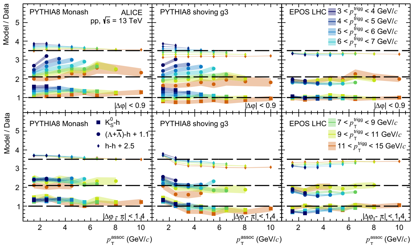
Fig. 7 Models to data ratio of integrated per-trigger yields for minimum bias collisions as a function of p_T^{\text{assoc}} for different p_T^{\text{trig}} intervals on the near-side (top panels) and away-side (bottom panels) for three MC models: PYTHIA8 Monash with colour re-connection (left),
