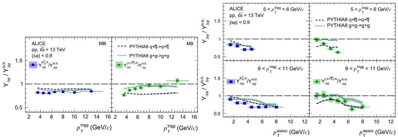
Fig. 10 Per-trigger yield ratios of K_S^0 -h (left column) or (\Lambda + \bar{\Lambda}) -h (right column) to h-h at the near-side as a function of p_T^{\text{trigg}} in the left plot and as a function of p_T^{\text{assoc}} in the right plot, compared with the PYTHIA8
