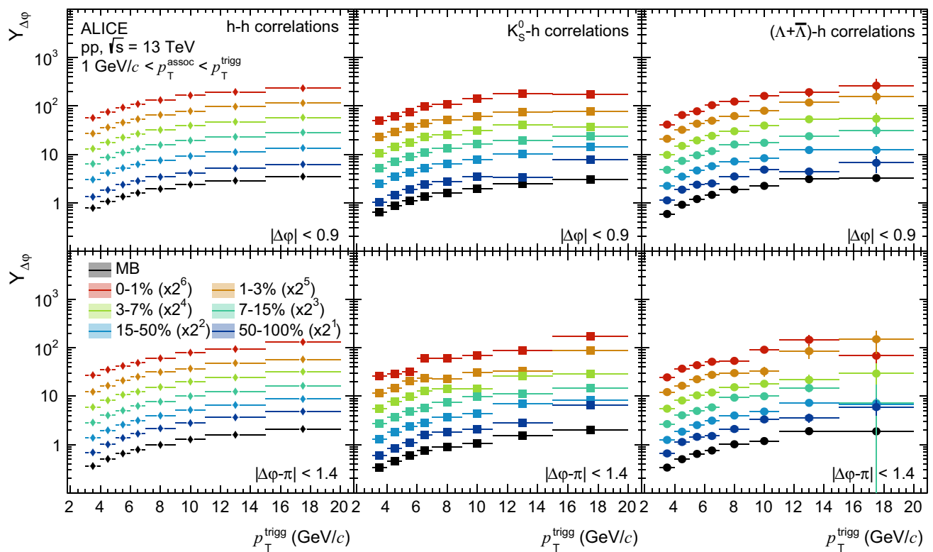
Fig. 3 Per-trigger yields of h-h (left), K_S^0 -h (middle) and (\Lambda + \bar{\Lambda}) -h (right) correlation functions as a function of p_T^{\text{trigg}} on the near-side (upper row) and away-side (lower row) for different multiplicity classes. For visibility, the values in the various event classes are scaled with the factors indicated in the legend. Error bars and colored boxes represent statistical and systematic uncertainties, respectively, which are in most cases within the data points
