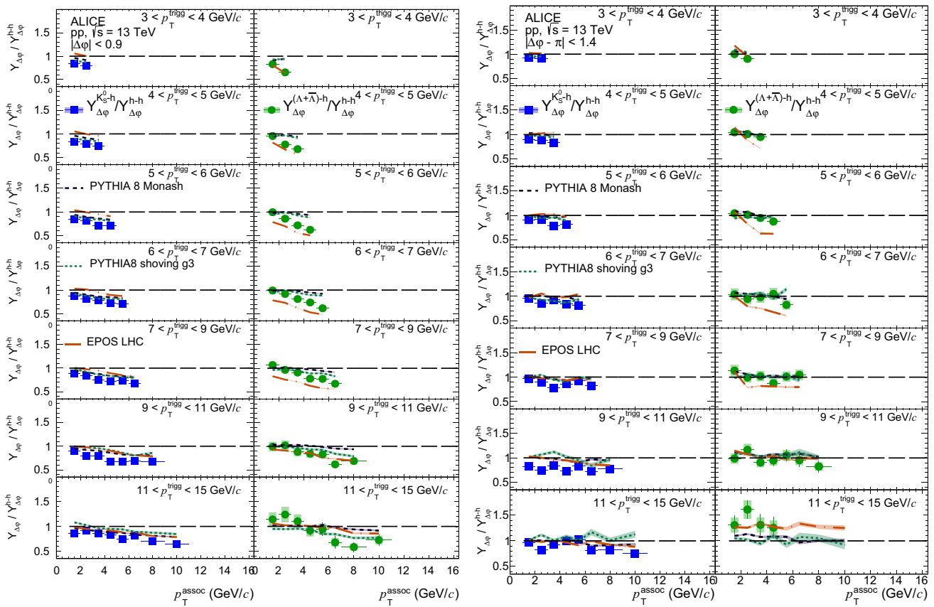
Fig. 9 Per-trigger yield ratios of K_S^0 -h (left column) or (\Lambda + \bar{\Lambda}) -h (right column) to h-h as a function of p_T^{\text{assoc}} , for the near-side in the left plot and for the away-side in the right plot, for different p_T^{\text{trigg}} intervals
