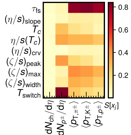
FIG. 18. Sensitivity of the mean multiplicity yields and mean transverse momenta ( p_T ) to the model parameters.
