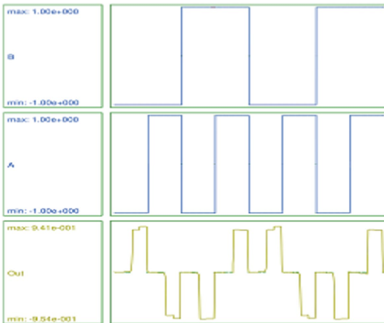
Fig. 12 The simulation result of the proposed design of QCA XNOR
