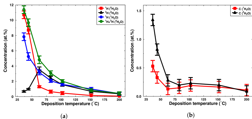
Figure 5. (a) Hydrogen isotope and (b) carbon concentration of the films deposited at different temperatures using 150 ms DEZ and 500 ms 1 H 2 O or 2 H 2 O pulses. Purging times after the precursor pulses were 10 and 20 s, respectively.
