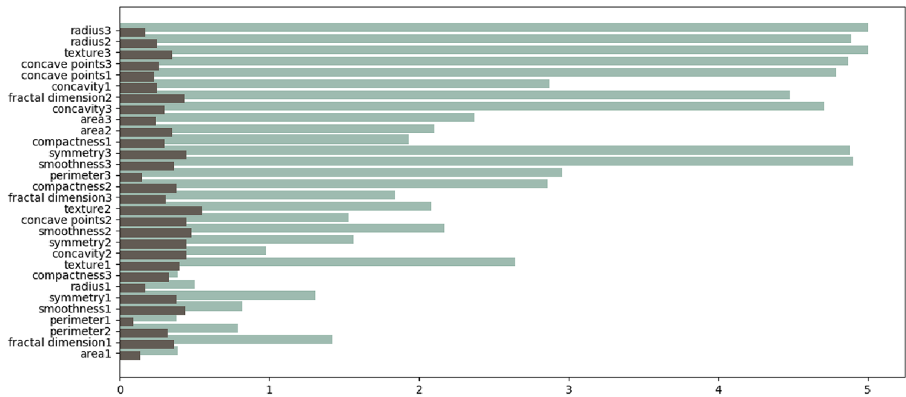
Fig. 3 Modular global feature importance values showing the average of how often (i.e., in each of the 5 folds within the 100 repetitions) a feature was selected by the L1 regularized logistic model for the breast cancer data. Light bars correspond to the results with
