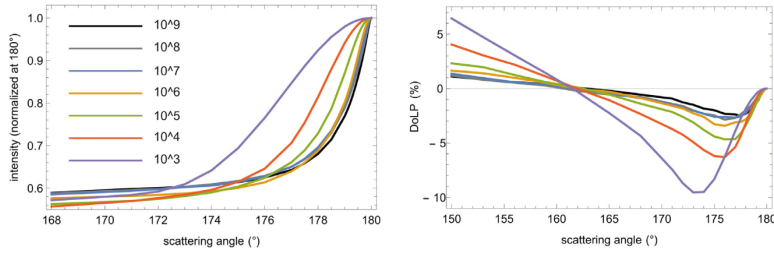
Fig. 5. The scattering phase function (in the left) and the degree of linear polarization (in the right) for backscattering region. Results are computed with the RT-CB-ic method. The plot legend panel indicates the powers of ten for the number of particles in the target.
