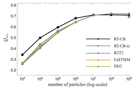
Fig. 4. The backscattering hemisphere scattering efficiency Q_{\text{bsca}} as a function of the target size, expressed as the number of the particles in the cloud. The Q_{\text{bsca}} is shown here for five methods, of which the FaSTMM and DEC rigorously solve the macroscopic Maxwell equations, and the RT-CB, RT-CB-ic, and R^2T^2 are based on the radiative transfer approximation. The results with ADDA go up to 10^5 particles and MSTM to 10^3 particles, they follow the same overall trend but are not shown here.
