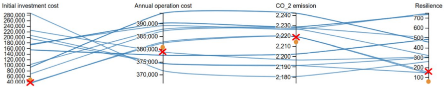
Fig. 4 Solutions after the second interaction of interactive K-RVEA. The orange dots are the aspiration levels forming the second reference point, and the red crosses are the aspiration levels forming the third reference point
