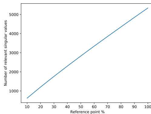
Figure 1. Mean of the number of relevant singular values in matrix \mathbf{D}_x as the function of reference points with dataset Computer Activity.
