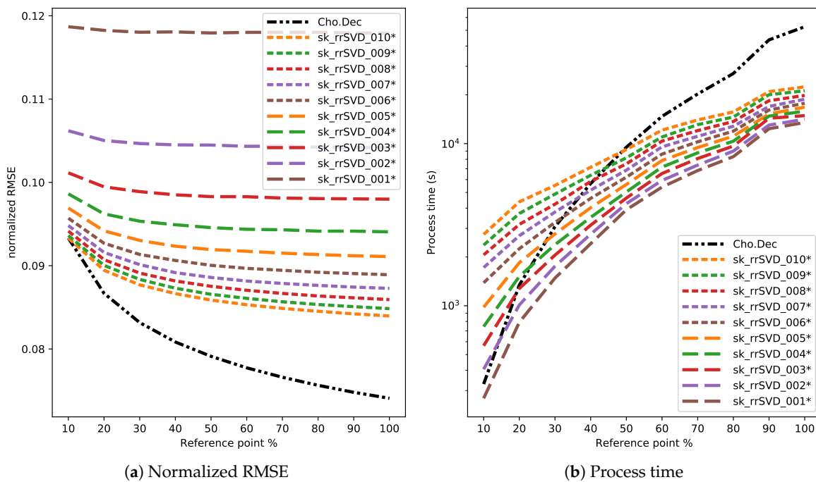
Figure 6. Normalized RMSE values (a) and process time in seconds taken to compute Equation (1) (b) as a function of reference point percentage for the Mnist dataset. Variants of sk_rrSVD_XX that differ statistically from Cholesky decomposition are marked with *.
