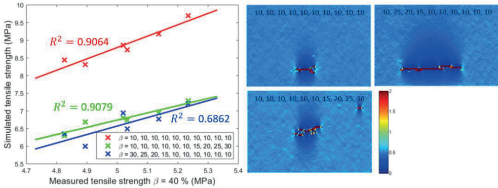
Figure 7.15. The effect of the through thickness moisture content distribution on the simulated fracture. The numbers in legends represent the moisture content ( \beta ) of the layers from bottom side to top side. Left: Correlations between measured and simulated MD tensile strengths. Right: Example of fracture initiation presented by MD strain (%) images. The MD is parallel to the vertical direction.
