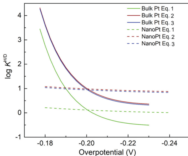
Fig. 6 \log K^{\text{H/D}} –overpotential diagrams for ORR with different analytical equations. The solid and dotted lines respectively indicate bulk Pt and nano Pt electrodes. The different features in bulk Pt and nano Pt electrodes are obtained. This can suggest a size-dependent quantum-to-classical transition in electrode processes. The figure was adopted with permission from the ref. 92. Copyright (2020) Royal Society of Chemistry.
