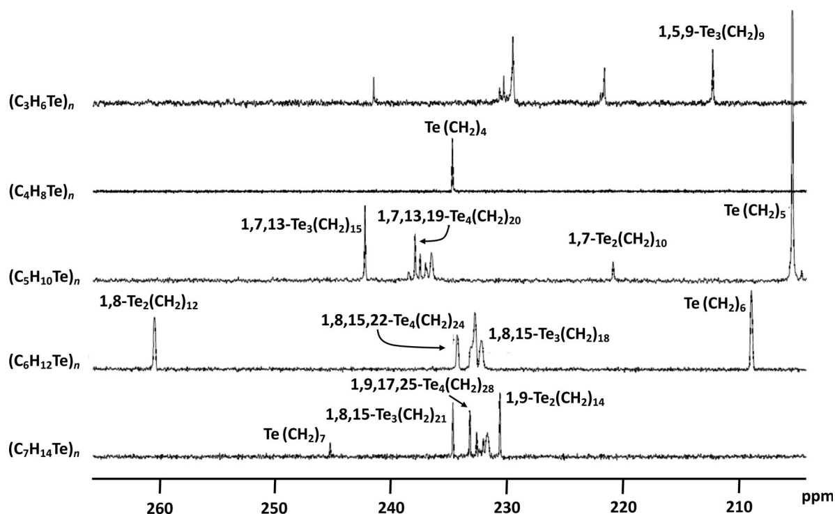
Figure 1. ^{125}\text{Te}\{^1\text{H}\} NMR spectra of the product mixtures of the reactions of \text{Na}_2\text{Te} and \text{Br}(\text{CH}_2)_m\text{Br} ( m=3-7 ). The peak of \text{Te}(\text{CH}_2)_5 was cut off at 43% of its height for better visibility of other reaction products. The partial assignment of the ^{125}\text{Te} resonances is based on the spectroscopic information of the isolated species (see Supporting Information).
