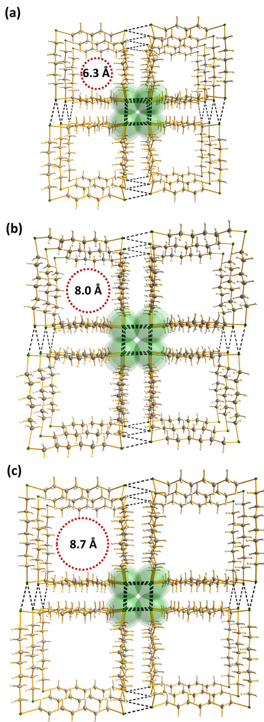
Figure 14. The pore openings in a) 1,7,13,19- \text{Te}_4(\text{CH}_2)_{20} , b) 1,8,15,22- \text{Te}_4(\text{CH}_2)_{24} and c) 1,9,17,25- \text{Te}_4(\text{CH}_2)_{28} . Te is depicted in green and C in grey.
