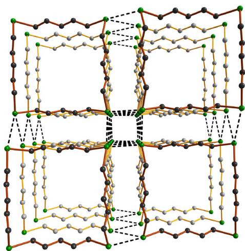
Figure 9. The \text{Te}\cdots\text{Te} close contacts form infinite rectangular shafts, as illustrated for 1,7,13,19- \text{Te}_4(\text{CH}_2)_{20} in two perpendicular views. The hydrogen atoms have been omitted for clarity. Te is depicted in green and C in grey.
