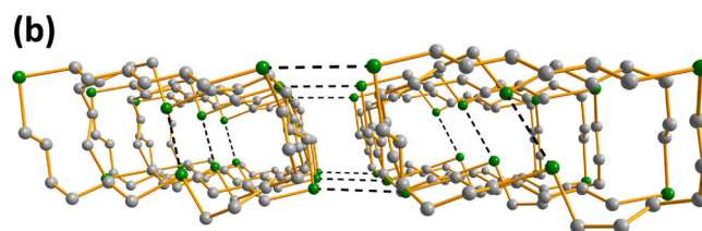
Figure 8. The tubular stacking of molecules of a) 1,5,9- \text{Te}_3(\text{CH}_2)_9 and b) 1,8,15- \text{Te}_3(\text{CH}_2)_{18} in the crystalline lattice. The hydrogen atoms have been omitted for clarity. Te is depicted in green and C in grey.
