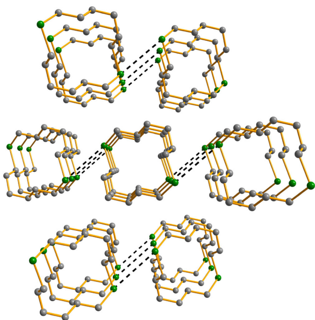
Figure 7. Tubular stacking of the 1,8- \text{Te}_2(\text{CH}_2)_{12} molecules in the crystal lattice. The hydrogen atoms have been omitted for clarity. Te is depicted in green and C in grey.
