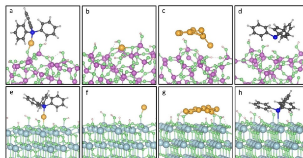
Figure 3. Lowest energy geometries obtained from DFT for different species on hydroxylated amorphous silica and hydroxylated ceria (111) surfaces. (a)–(d) AuL and Au 9 species formed by oxidative fragmentation, and Au 9 and L formed by ligand migration, respectively on the SiO 2 surface. (e)–(h) AuL and Au 9 species formed by oxidative fragmentation, and Au 9 and L formed by ligand migration, respectively on the CeO 2 surface. Au, P, C, O, Si and Ce are shown by yellow, blue, dark grey, pale green, pink and pale blue colours, respectively. H atoms in the phenyl ring and on the surface hydroxyl groups are shown by light grey and light pink colours, respectively.
