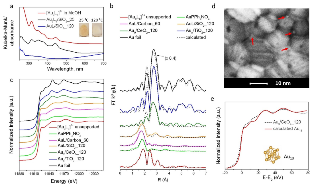
Figure 2. (a) UV/Vis of the unsupported [\text{Au}_9\text{L}_8]^{3+} in methanol, DR UV/Vis and photographs (inset) of \text{Au}_9\text{L}_8/\text{SiO}_2_{25} and \text{AuL}/\text{SiO}_2_{120} . (b) FT of Au L_{III} EXAFS (uncorrected for the phase shift) and (c) Au L_{III} XANES of supported [\text{Au}_9\text{L}_8]^{3+} (at total Au loading 0.2 wt.%, see Table 3) after thermal treatment and reference compounds. FT EXAFS intensity of Au foil was reduced 2.5 times to fit in the Figure. (d) HAADF-STEM of \text{Au}_9/\text{CeO}_2_{120} . Au nanoclusters are seen as white dots. (e) Experimental Au L_{III} XANES of \text{Au}_9/\text{CeO}_2_{120} and calculated XANES of \text{Au}_{13} .
