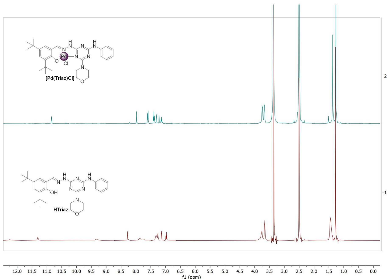
Fig. 3. ^1\text{H} NMR spectra of ( HTriaz ) and [Pd(Triaz)Cl] in \text{DMSO-}d_6 .
