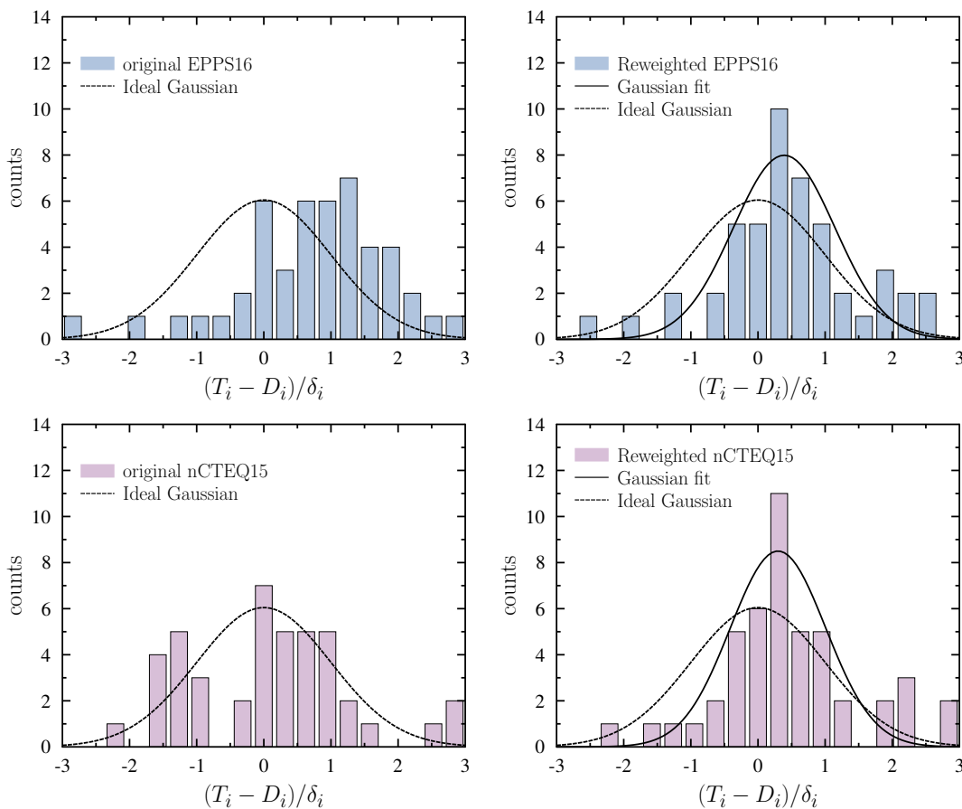
Figure 5. The histograms of the R_{pPb}^{D0} -data residuals obtained before (left) and after (right) the reweighting with EPPS16 (top) and nCTEQ15 (bottom). Ideal Gaussian distributions (dashed) are compared to fitted ones (solid) in the reweighted case.
