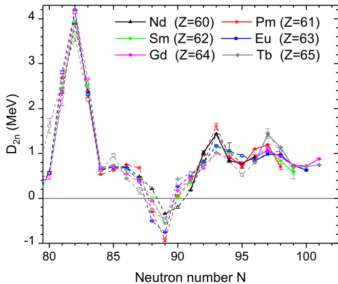
FIG. 13. D_{2n} values based on the AME16 [21] experimental mass values (dashed lines and open symbols) and the JYFLTRAP mass measurements from this work and Ref. [26] (thick solid lines and full symbols). No subshell at N = 100 is apparent but two peculiar peaks appear at N = 93 and N = 97 .
