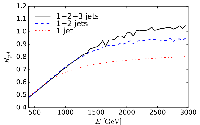
FIG. 4. Nuclear modification factor for the jet-energy spectrum in CASTOR kinematics at \sqrt{s} = 5.02 TeV including contributions from up to three merged jets. The proton-proton reference is computed with the same kinematical shift as applied in the proton-nucleus scattering.
