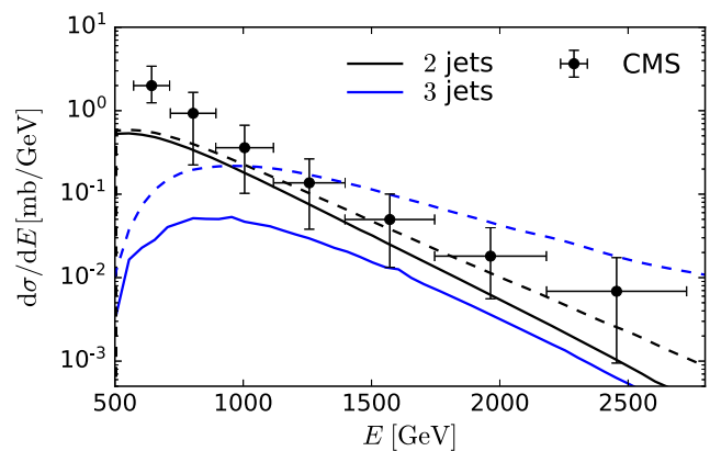
FIG. 9. Contribution on the jet-energy spectra from two merged jets (black lines) and three merged jets (blue lines) in proton-nucleus collisions at \sqrt{s} = 5.02 TeV. Solid lines include the kinematical constraint, and dashed lines do not.
