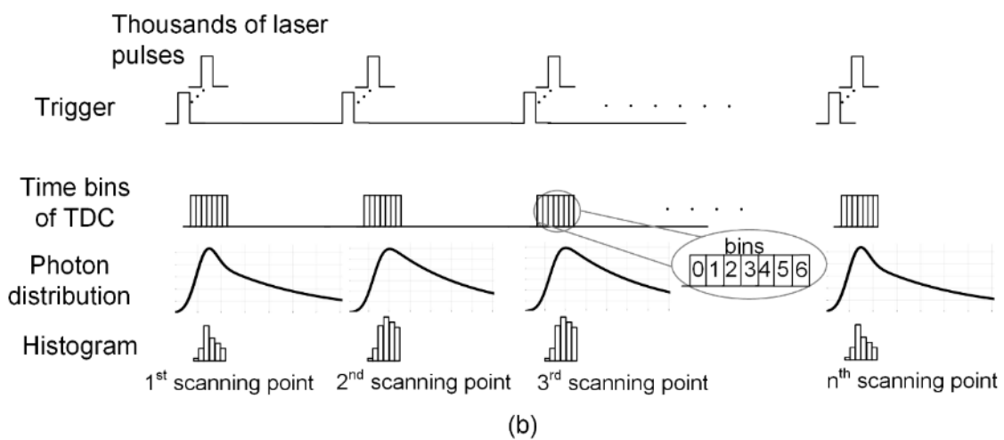
Figure 2. a) Block diagram of time-gated Raman spectrometer and b) timing diagram of the operation of a single spectral point in sample scanning.
