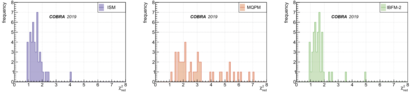
Fig. 6. Distribution of the minimum \chi_{\text{red}}^2 values of the 45 best match g_A values for the single detector spectrum shape comparison.
