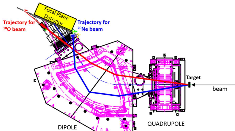
Fig. 1. Drawing of the MAGNEX spectrometer showing two typical trajectories of the ^{18}\text{O} and ^{20}\text{Ne} beams in the experimental conditions used for the DCE measurements.
