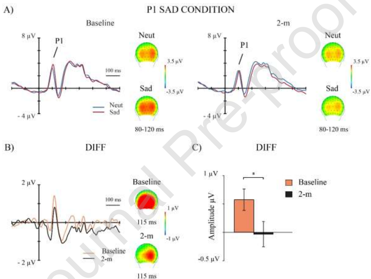
Fig. 6. The grand-averaged P1 responses in the Sad condition for the depressed group (n = 25) at the baseline measurement and at the 2-m measurement. A) The waveforms averaged for the left and right occipital electrode cluster and the topographical maps of the P1 responses (mean amplitude value at 80-120 ms after stimulus onset) to the sad faces and the neutral faces preceding the sad face (neut). B) Differential waveforms (Diff; sad minus neutral) and the topography of the differential responses (peak value at 115 ms after stimulus onset) at the
