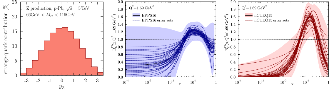
Figure 2: Left: Percentual contribution of s\bar{s} scattering to Z production at \sqrt{s} = 5 TeV. Middle: The EPPS16 gluon nuclear modifications with individual error sets at Q^2 = 1.69 \text{ GeV}^2 . Right: The nCTEQ15 gluon nuclear modifications with individual error sets at Q^2 = 1.69 \text{ GeV}^2 .
