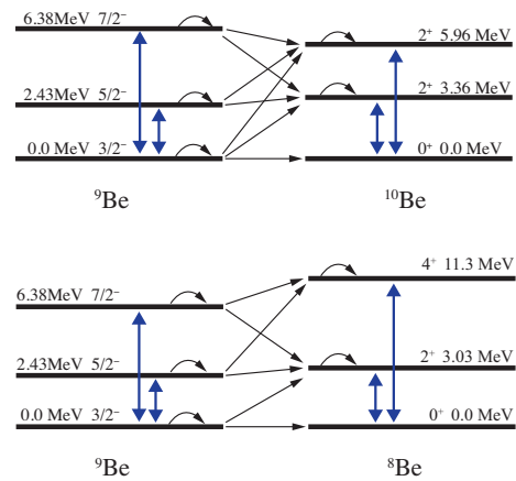
Figure 5. The target coupling schemes in the {}^9\text{Be}(d, p){}^{10}\text{Be} (upper) and the {}^9\text{Be}(d, t){}^8\text{Be} (lower) nuclear reactions. The bold two-headed arrows indicate E1 transitions. The spin reorientation effects are indicated as back-pointing arrows.
