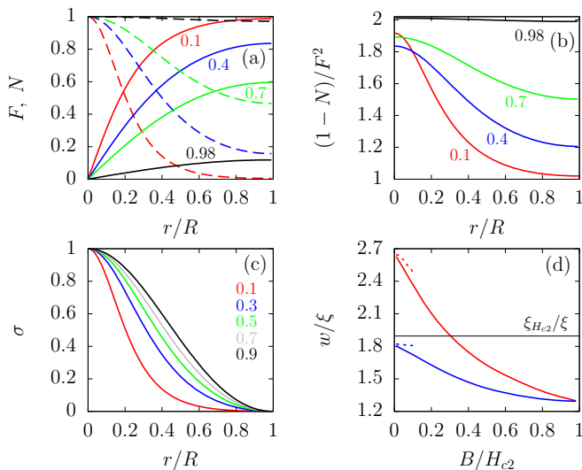
FIG. 1. Vortex structure in the single-band model at T/T_c = 0.05 . (a) Normalized gap distribution (solid curves) inside the vortex cell, F = |\Delta|/\Delta_0 . Numbers near each curve indicate the value of B/H_{c2} . The dashed curves with the same color show zero-energy LDOS N . (b) Proportionality coefficient between 1 - N and F^2 within the vortex cell for different magnetic fields. Note that we obtain (1 - N)/F^2 = 2 near H_{c2} , in agreement with Eq. (1). (c) LDOS variation \sigma = \delta N(r)/\delta N(0) for different ratios B/H_{c2} . (d) The field behavior of the vortex-core size w = w_\Delta determined by the half-width of the squared gap |\Delta|^2 (red curve) and the w = w_\sigma one defined by the half-width of the LDOS variation \sigma (blue curve). Both quantities are shown in units of \xi = \sqrt{D/(2\pi T_c)} . The dashed curves are calculated by means of Eq. (2) with substitution \hat{\nabla} \rightarrow \nabla (see discussion in the text). The black horizontal line is the length scale determined by the upper critical field, \xi_{H_{c2}} = \sqrt{\phi_0/(2\pi H_{c2})} .
