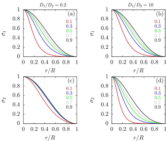
FIG. 4. LDOS variations \sigma_k = \delta N_k(r)/\delta N_k(0) inside the vortex as the value of the normalized magnetic field B/H_{c2} , indicated by different colored lines, increases. Left and right columns correspond to the cases D_1/D_2 = 0.2, 10 , respectively.
