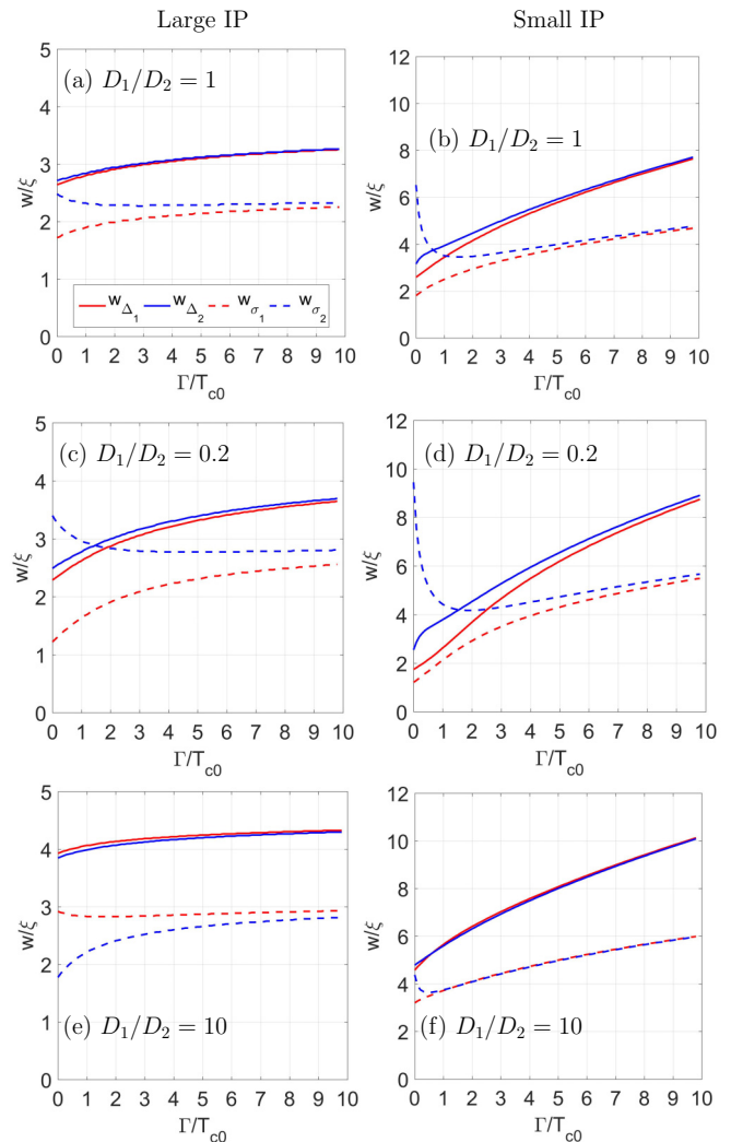
FIG. 6. Dependencies of different vortex-core sizes on the interband scattering rate for the case of (a), (c), and (e) large interband pairing (IP) \lambda_{12} = 0.0336 , \lambda_{21} = 0.0264 and (b), (d), (f) small IP \lambda_{12} = 0.00336 , \lambda_{21} = 0.00264 parameters as defined in the text. Different ratios of diffusion coefficients in the two bands are considered. The temperature is T = 0.1T_{c0} .
