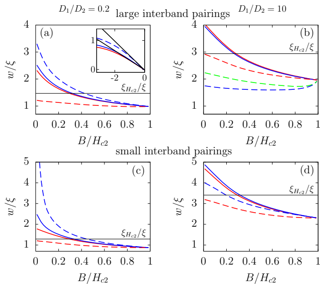
FIG. 5. Field dependence of the length scales normalized to \xi = \sqrt{\sqrt{D_1 D_2}/(2\pi T_c)} for D_1/D_2 = 0.2, 10 (left and right columns, respectively). Red and blue solid lines correspond to strong and weak band lengths w = w_{\Delta_{1,2}} determined as the half-widths of |\Delta|_{1,2}^2 , and red and blue dashed lines correspond to w = w_{\sigma_{1,2}} defined as the half-widths of \sigma_{1,2} , respectively. The black horizontal line is the length scale determined by the upper critical field, \xi_{H_{c2}} = \sqrt{\phi_0/(2\pi H_{c2})} . (a) and (b) Large interband pairings; (c) and (d) small interband pairings. The inset in (a) shows a logarithmic-scale plot of w_{\Delta_{1,2}}(B) (red and blue solid curves) and w_{\sigma_2}(B) (blue dashed curve). Linear dependencies y = -x/2 + \text{const} (upper black curve) and y = -x/3 + \text{const} (lower black curve) indicate the scalings w_{\sigma_2} \sim (B/H_{c2})^{-1/2} and w_{\Delta_{1,2}} \sim (B/H_{c2})^{-1/3} for a wide range of fields. The green dashed curve in (b) is the half-width of the total LDOS, (N_1 + N_2)/2 .
