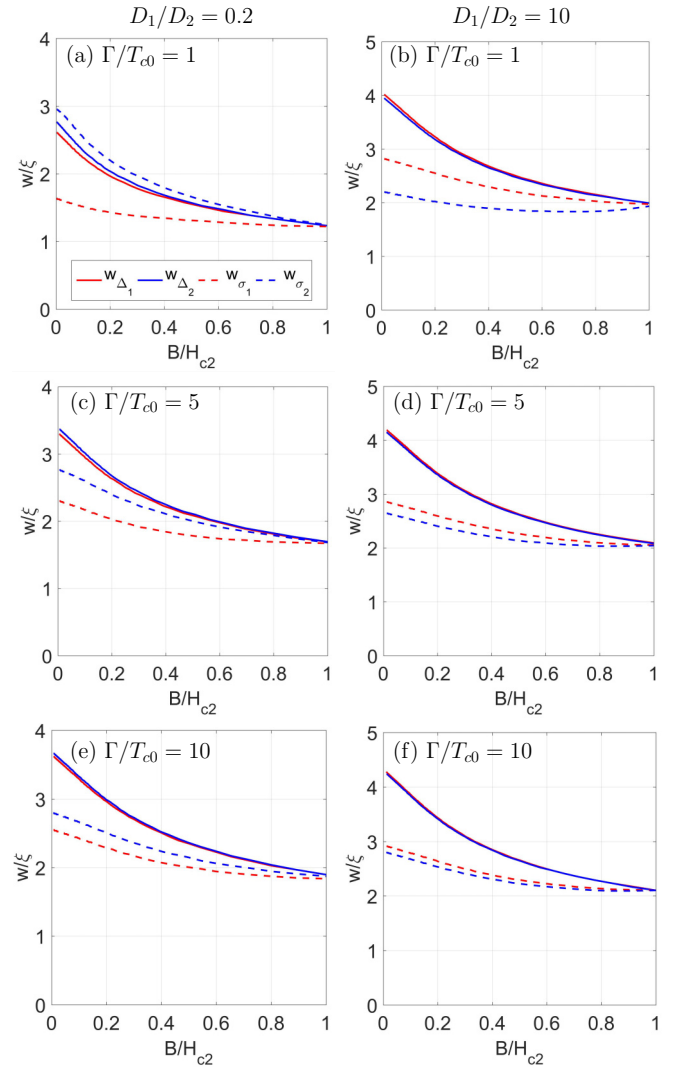
FIG. 7. Field dependencies of vortex-core sizes for different interband scattering rates and the ratios of diffusion constants (a), (c), and (e) D_1/D_2 = 0.2 and (b), (d) and (f) D_1/D_2 = 10 . The interband pairing constants are \lambda_{11} = 0.1012 , \lambda_{22} = 0.0448 , \lambda_{12} = 0.0336 , \lambda_{21} = 0.0264 . The temperature is T = 0.1T_{c0} .
