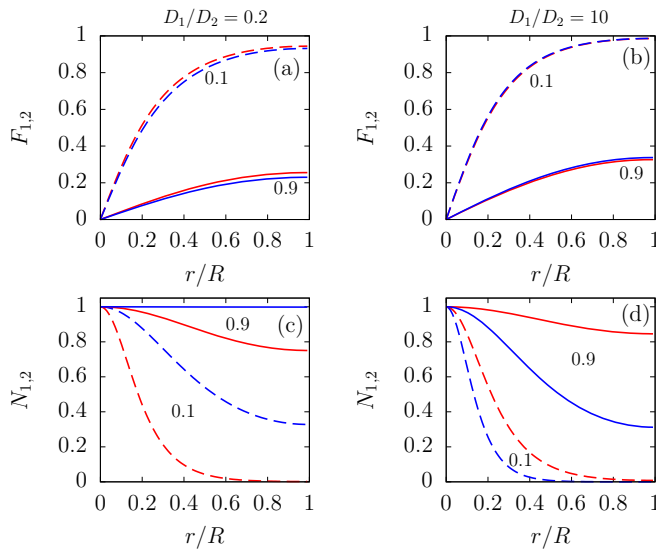
FIG. 2. Vortex structure in the two-band model at T/T_c = 0.1 for D_1/D_2 = 0.2, 10 (left and right columns, respectively). (a) and (b) Gap profiles in each band normalized by the bulk value, F_k = |\Delta_k|/\Delta_{k0} . Red and blue curves correspond to strong and weak bands F_1 and F_2 , respectively. Dashed curves are for B/H_{c2} = 0.1 , and solid curves correspond to B/H_{c2} = 0.9 . (c) and (d) LDOS in each band N_k for small (dashed curve) and high (solid curve) fields. Red and blue curves correspond to weak and strong bands N_{1,2} , respectively.
