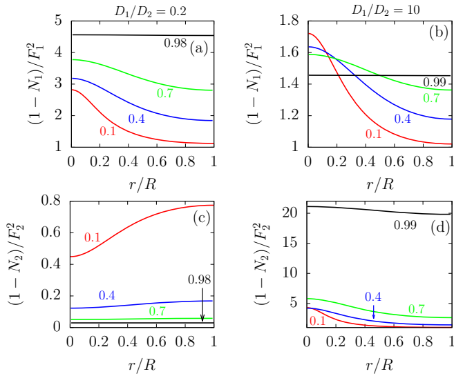
FIG. 3. Spatial variation of the proportionality coefficient between 1 - N_k and F_k^2 in the two-band model with D_1/D_2 = 0.2, 10 (left and right columns, respectively). (a) and (b) Coefficient for the stronger-superconductivity band as B/H_{c2} , indicated by the colored numbers, increases. (c) and (d) Coefficient for the weaker-superconductivity band.
