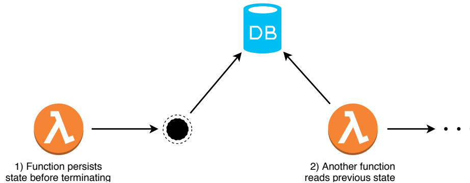
Figure 12: Externalized State
