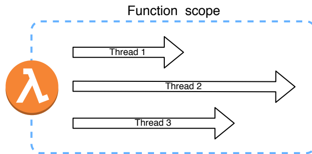
Figure 34: Local Threader
