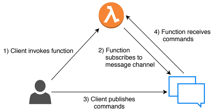
Figure 33: Task Controller
