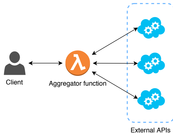
Figure 19: Aggregator
