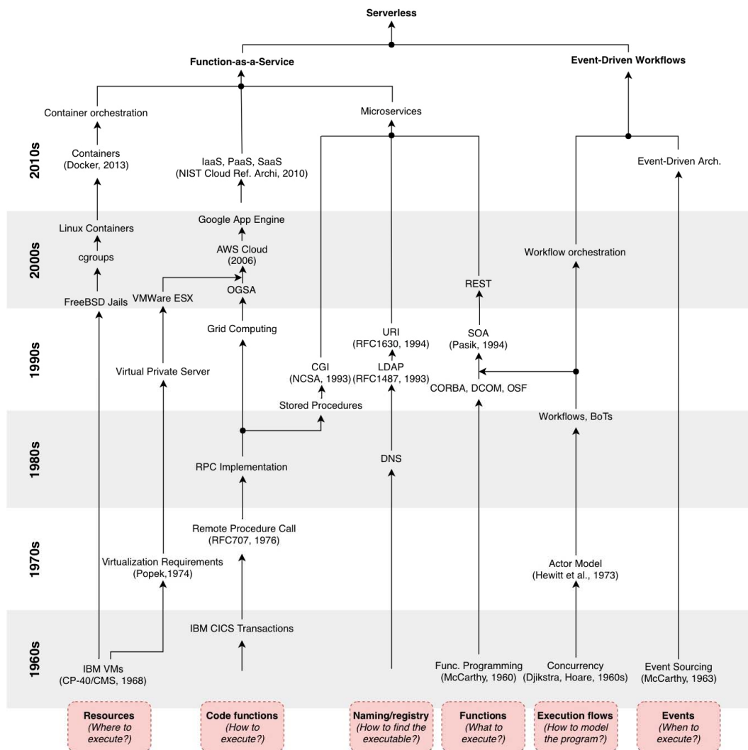
Figure 2: A history of computer science concepts leading to serverless computing (Eyk, Toader, et al. 2018)
