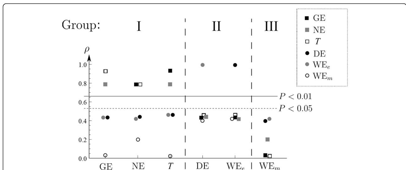
Fig. 1 Spearman's rank correlations \rho for the inspected six indices of mechanical efficiency. With two transversal lines, values corresponding to significance levels p < 0.05 and p < 0.01 have been drawn. The indices can be divided into three groups: groups I, II, and III. GE gross efficiency, NE net efficiency, T economy, DE delta efficiency, WE_e work efficiency with extrapolated zero load energy expenditure, WE_m work efficiency with measured zero load energy expenditure
