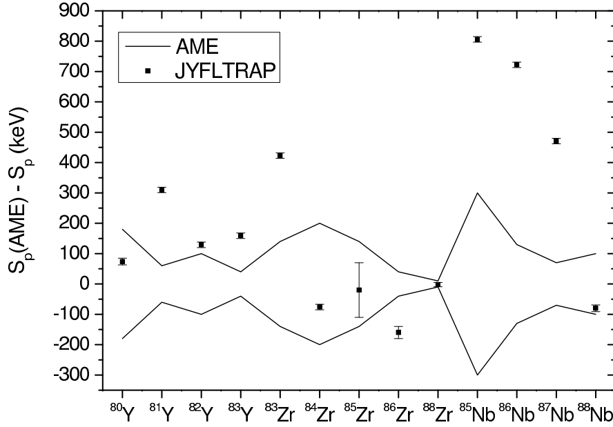
Fig. 9. Proton separation energies for the measured nuclides relative to AME values. The two lines show the corridor of uncertainties taken from ref. [14]. The mass of the (Z-1,N) nucleus is from this experiment for ^{83}\text{Zr} , ^{84}\text{Zr} , ^{85}\text{Nb} , ^{86}\text{Nb} and ^{87}\text{Nb} . For the others, the AME mass [14] of the (Z-1,N) nucleus has been used.
