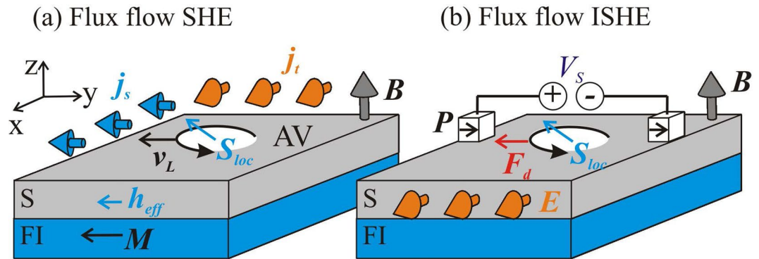
Figure 1. The mechanisms of direct and inverse flux-flow spin Hall effects. The schematic picture of (a) flux-flow spin Hall effect (SHE) and (b) flux-flow inverse spin Hall effect (ISHE) in type-II superconductors. Magnetic field \mathbf{B} perpendicular to film plane creates Abrikosov vortices (AV). Vortex cores contain localized spin polarization \mathbf{S}_{loc} due to the splitting field \mathbf{h} = \mathbf{h}_{eff} + \mu_B \mathbf{B} . (a) Transport current \mathbf{j} = \mathbf{j}_t generates the Lorentz force driving motion of spin-polarized AV with the velocity \mathbf{v}_L \perp \mathbf{j} and inducing the spin current \mathbf{j}_s \parallel \mathbf{v}_L . (b) Ferromagnetic electrodes with polarization \mathbf{P} generate spin-dependent bias V_s . The induced spin accumulation gradient \nabla \mu_s produces the driving force on AV, \mathbf{F}_d \parallel \nabla \mu_s which results in the AV motion in the direction \mathbf{v}_L \parallel \nabla \mu_s and induction of the average electric field \mathbf{E} = \mathbf{B} \times \mathbf{v}_L .
