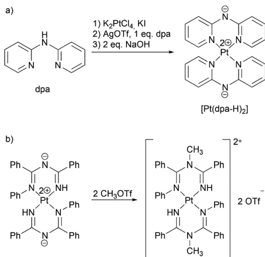
Scheme 3 Known reactions of platinum(II) complexes, which inspired this work: (a) synthesis of [\text{Pt}(\text{dpa-H})_2] , 23 (b) methylation of [\text{Pt}(\text{NH}=\text{C}(\text{Ph})_2)_2] . 26
