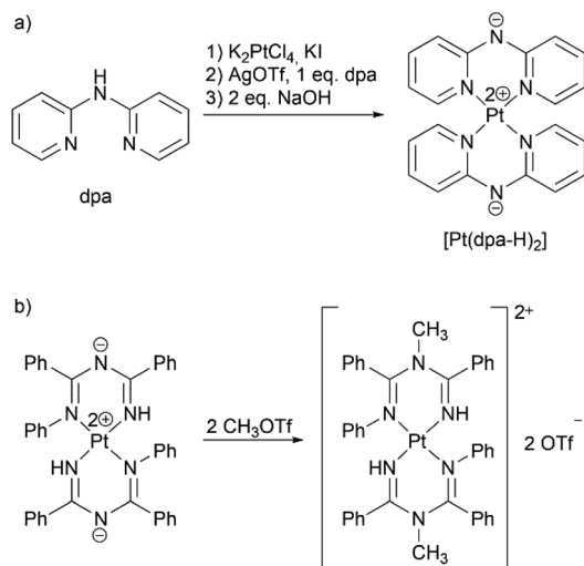
Scheme 3 Known reactions of platinum(II) complexes, which inspired this work: (a) synthesis of [\text{Pt}(\text{dpa-H})_2] , 23 (b) methylation of [\text{Pt}(\text{NH}=\text{NC}(\text{Ph})=\text{NPh})_2] . 26
