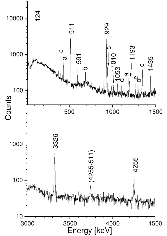
FIG. 1. Partial \gamma spectra taken in coincidence with \beta particles at A=34 . Peaks identified by their energy in keV are from the ^{34}\text{Al} beta decay. Those labeled by a letter are from the decay of (a) ^{34}\text{Si} , (b) ^{204}\text{At} ( 6^+ in A=34 ), (c) ^{28}\text{Mg} , (d) ^{116}\text{In} ( 4^+ in A=29 ), and (e) ^{29}\text{Al} .
