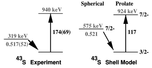
FIG. 11. First excited states in ^{43}\text{S} . Shell-model predictions are compared to experimental values (Refs. [4,5]); numbers next to the transitions are B(E2) values in units of e^2 \text{ fm}^4 .
