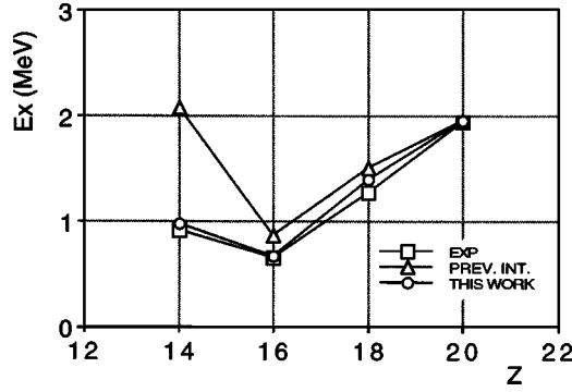
FIG. 10. Evolution of the (3/2)^- excitation energy in N=21 isotones. The experimental values (squares) are compared with two calculations using the set of parameters used for the interaction prior to this experiment (triangles), and the single-particle energy for Z=14 obtained in this work (circles).
