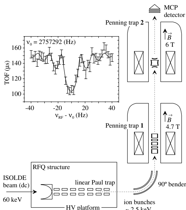
FIG. 1. Experimental setup of the ISOLTRAP mass spectrometer. The inset shows the cyclotron resonance curve for ^{33}\text{Ar} . The time of flight (TOF) of the ions from the trap to the ion detector is plotted as a function of the applied radio frequency \nu_{\text{rf}} . The solid line is a fit of the theoretical line shape [10] to the data points.
