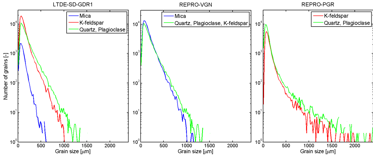
Fig. 7 Grain size distributions of the LTDE-SD-GDR1 (left column), REPRO-VGN (middle column), and REPRO-PGR (right column) samples. The distributions were determined from tomographic images with grains segmented, and the distributions are determined using 20 \mu\text{m} bin size.
