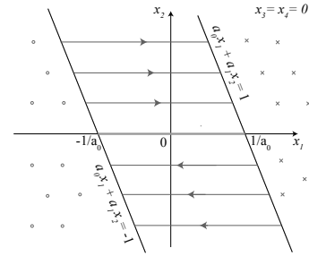
Fig. 1. Sliding mode manifold \{(x_1, x_2, x_3, x_4) \in \mathbb{R}^4 \mid x_3 = x_4 = 0, -1 \leq a_0x_1 + a_1x_2 \leq 1\} for the Fitts system (4). Arrowed lines define the motion on the surface, thick green line defines the rest segment.
