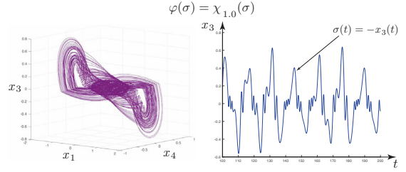
Fig. 5. Strange attractor in the system (4) for \beta = 0.1 and \varphi(\sigma) = \chi_\varepsilon(\sigma) \equiv \psi_N(\sigma) + \varepsilon(\tanh(\sigma/N) - \psi_N(\sigma)) , N = 0.01 , \varepsilon = 1 .
