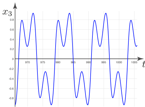
Fig. 8. Periodic solution of the system (4) for \beta = 0.03 .
