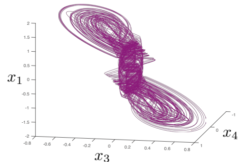
Fig. 7. Projection of the strange attractor in the system (4) for \beta = 0.1 in the subspace (x_1, x_3, x_4) .
