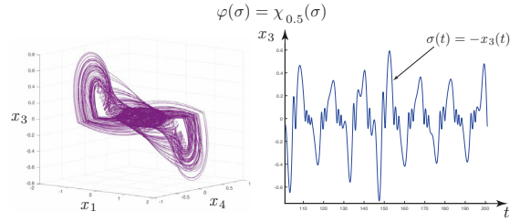
Fig. 4. Strange attractor in the system (4) for \beta = 0.1 and \varphi(\sigma) = \chi_\varepsilon(\sigma) \equiv \psi_N(\sigma) + \varepsilon(\tanh(\sigma/N) - \psi_N(\sigma)) , N = 0.01 , \varepsilon = 0.5 .
